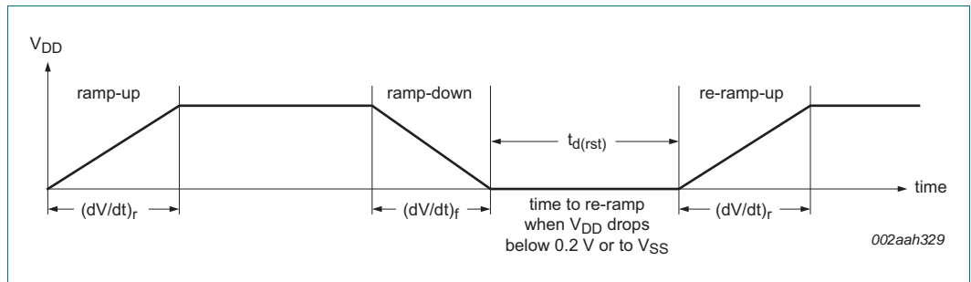
Fig 17. V DD is lowered below 0.2 V or 0 V and then ramped up to V DD
