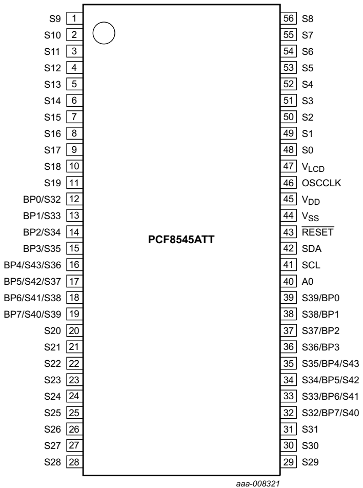
Fig 3. Pin configuration for TSSOP56 (PCF8545ATT)
