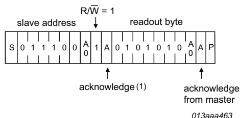
Fig 31. I 2 C-bus protocol read mode
