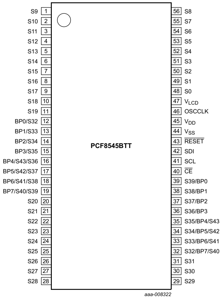
Fig 4. Pin configuration for TSSOP56 (PCF8545BTT)
