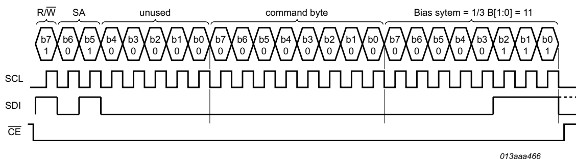
Fig 34. SPI-bus example
