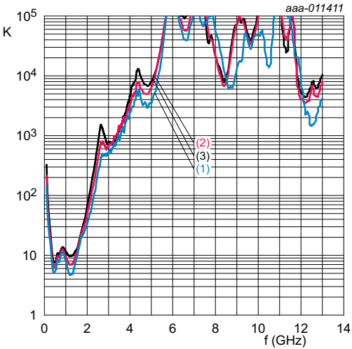
GS1 = HIGH; GS2 = LOW; V_{CC1} = 5\text{ V} ; V_{CC2} = 5\text{ V} ; V_{ctrl}(Gp) = 0\text{ V} . (1) T_{amb} = -40\text{ }^{\circ}\text{C} (2) T_{amb} = +25\text{ }^{\circ}\text{C} (3) T_{amb} = +85\text{ }^{\circ}\text{C}
