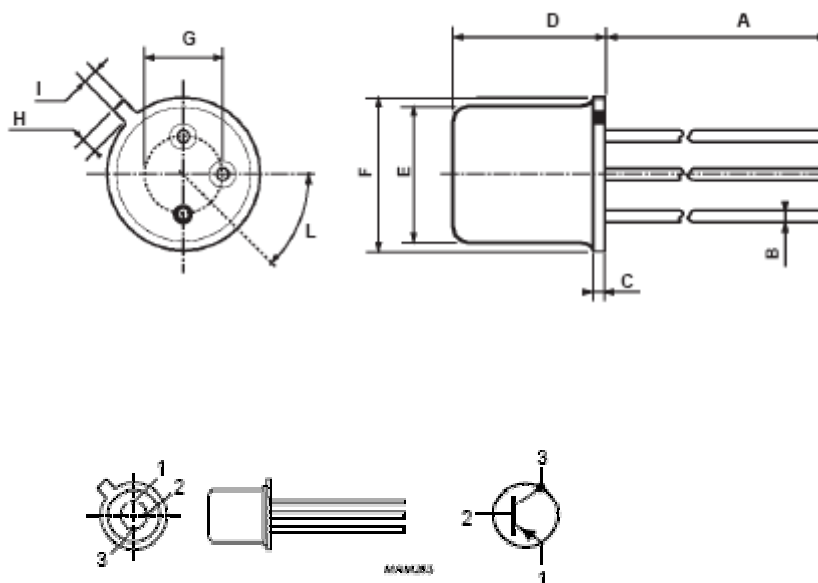
Fig.1 Simplified outline (TO-18) and symbol.
