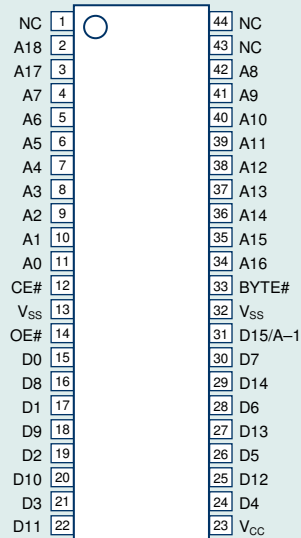
44SOP
