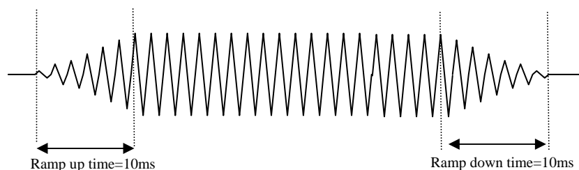
Figure 11 Pulse Metering Tone Waveform
