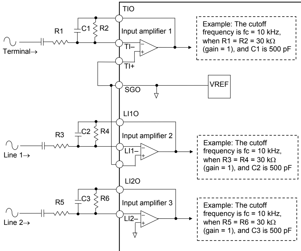
Figure 1 Input amplifier 1 to 3 interface
