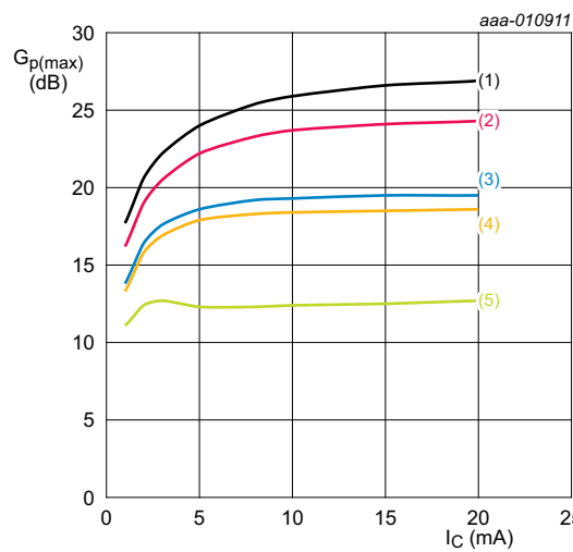
V_{CE} = 8\text{ V} ; T_{amb} = 25\text{ }^{\circ}\text{C} . If K > 1 then G_{p(max)} = maximum power gain. If K < 1 then G_{p(max)} = \text{MSG} . (1) f = 300\text{ MHz} (2) f = 433\text{ MHz} (3) f = 800\text{ MHz} (4) f = 900\text{ MHz} (5) f = 1800\text{ MHz}
