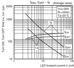
G3VM-355JR
