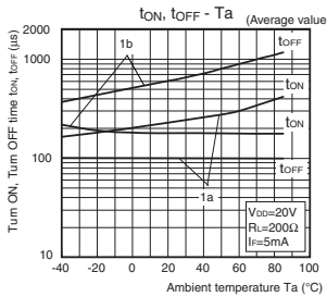
G3VM-355JR
