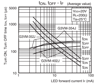
G3VM-352J/354J/402J
