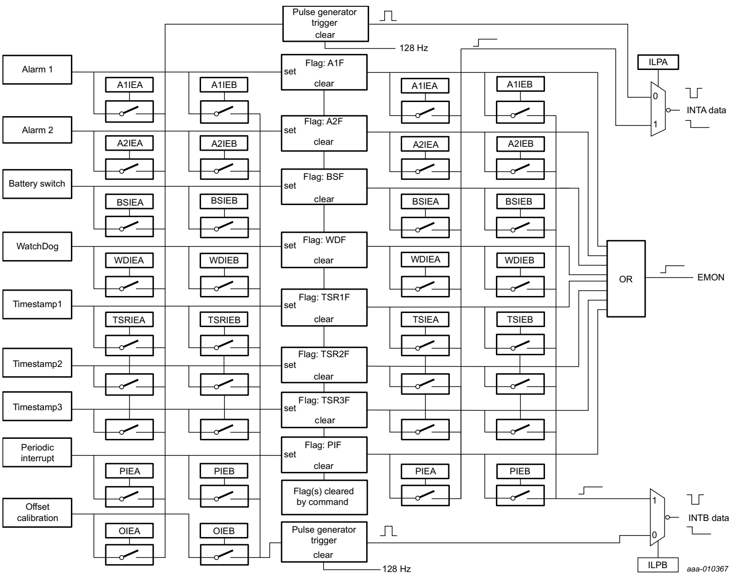
Fig 22. Interrupt selection
