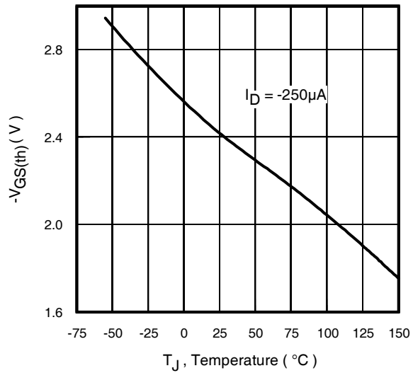
Fig 15. Typical Threshold Voltage Vs. Junction Temperature
