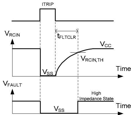
Figure 4: RCIN and FAULT pin waveforms
