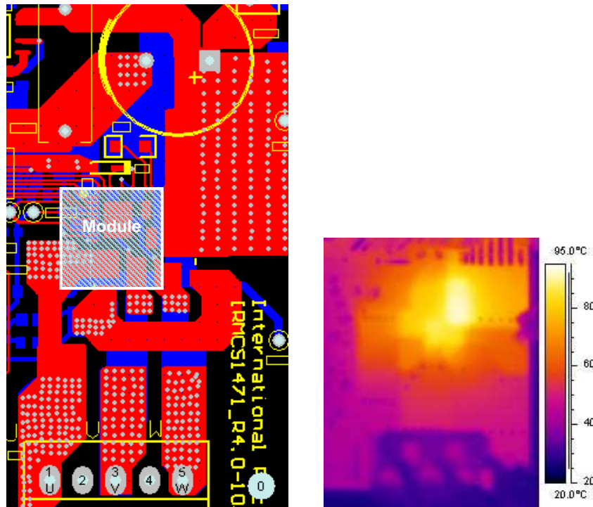
Figure 7: PCB layout example and corresponding thermal image (16kHz, 2P, 1oz, \Delta T_{ca}=70^{\circ}\text{C} , V_+ = 320\text{V} , I_u = 392\text{mA} , P_o = 88\text{W} )
