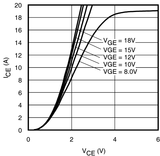
Fig. 7 - Typ. IGBT Output Characteristics T J = 150°C; t p = 60μs
