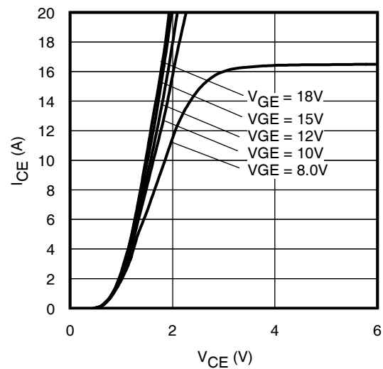
Fig. 6 - Typ. IGBT Output Characteristics T J = 25°C; t p = 60μs
