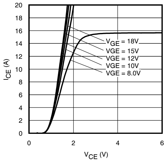
Fig. 5 - Typ. IGBT Output Characteristics T J = -40°C; t p = 60μs
