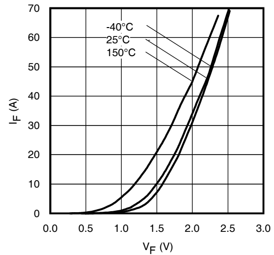
Fig. 8 - Typ. Diode Forward Characteristics t p = 60μs
