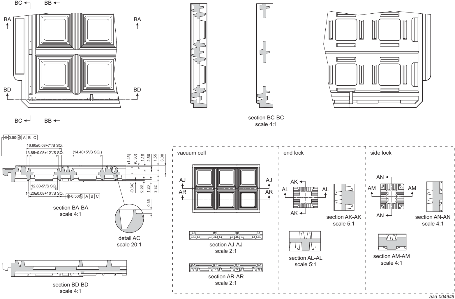
Fig 33. Tray details
