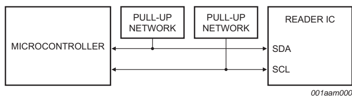
Fig 13. I 2 C-bus interface
