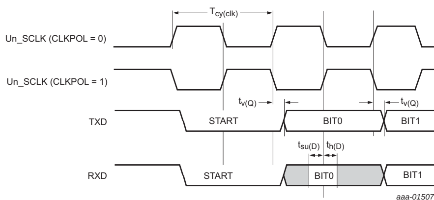
Fig 37. USART timing
