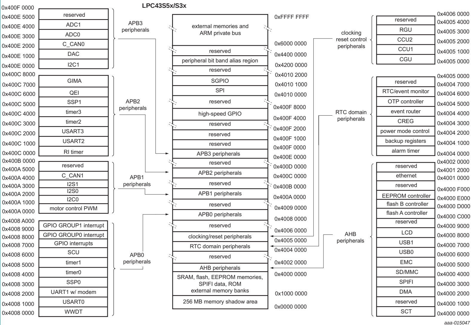
Fig 8. LPC43S5x/S3x Memory mapping (peripherals)
