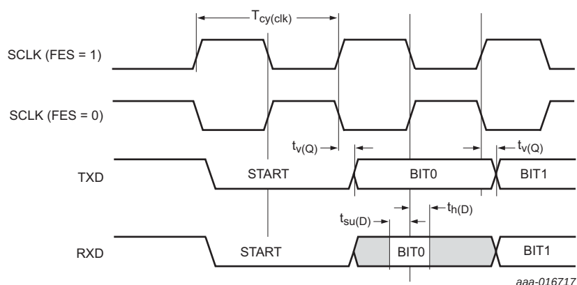
Fig 30. USART timing
