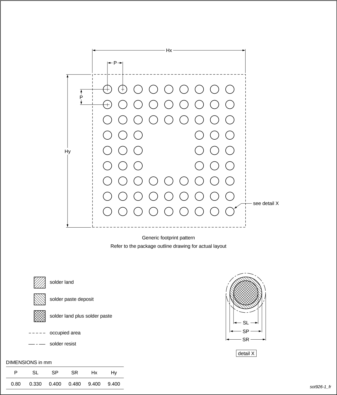
Fig 56. Reflow soldering of the TFBGA100 package
