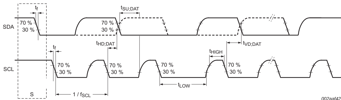
Fig 24. I 2 C-bus pins clock timing
