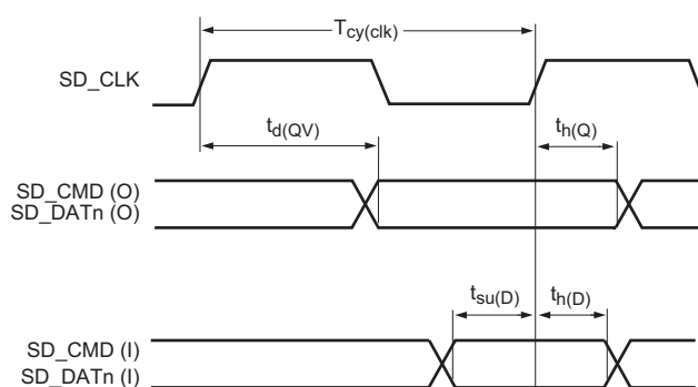
Fig 37. SD/MMC timing
