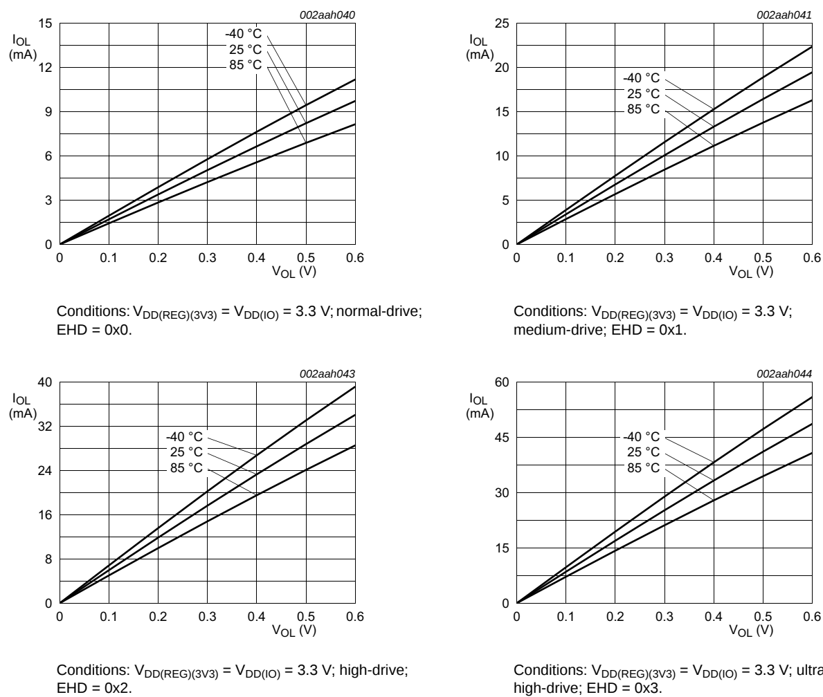
Fig 19. High-drive pins; typical LOW level output current I_{OL} versus LOW level output voltage V_{OL}
