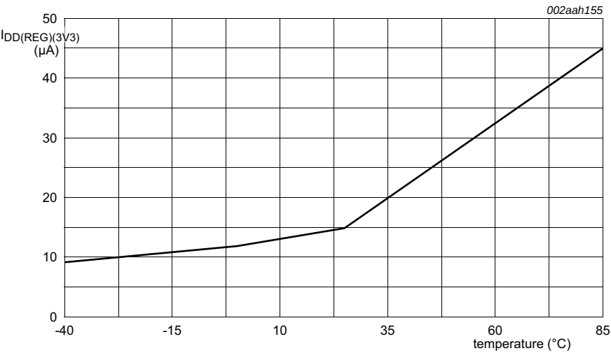
Fig 13. Typical supply current versus temperature in Power-down mode
