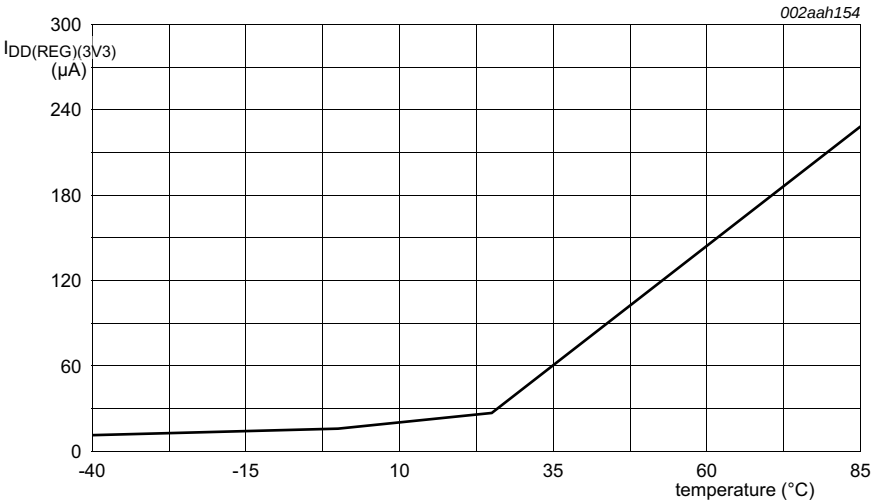
Fig 12. Typical supply current versus temperature in Deep-sleep mode
