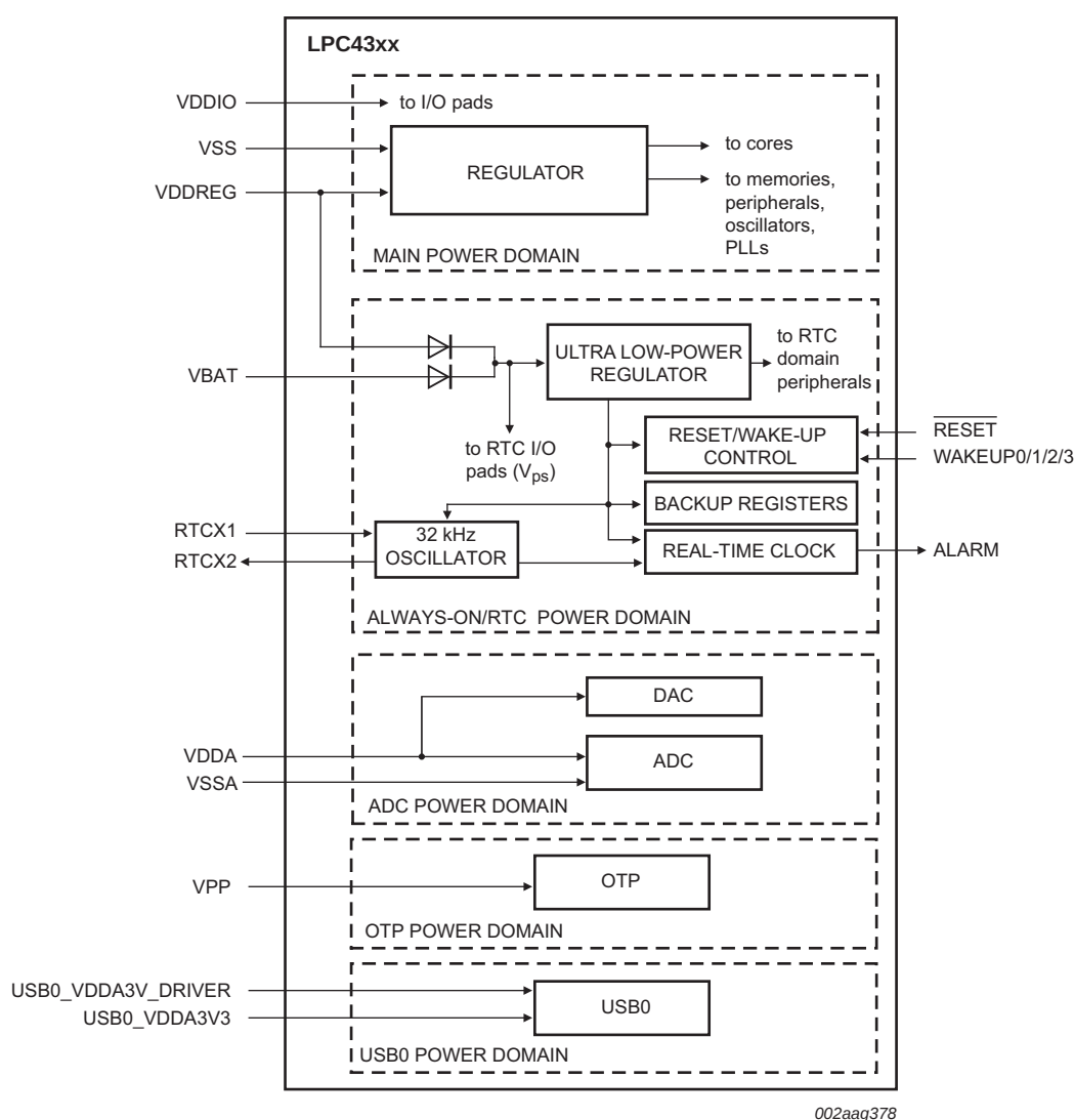
Fig 7. Power domains
