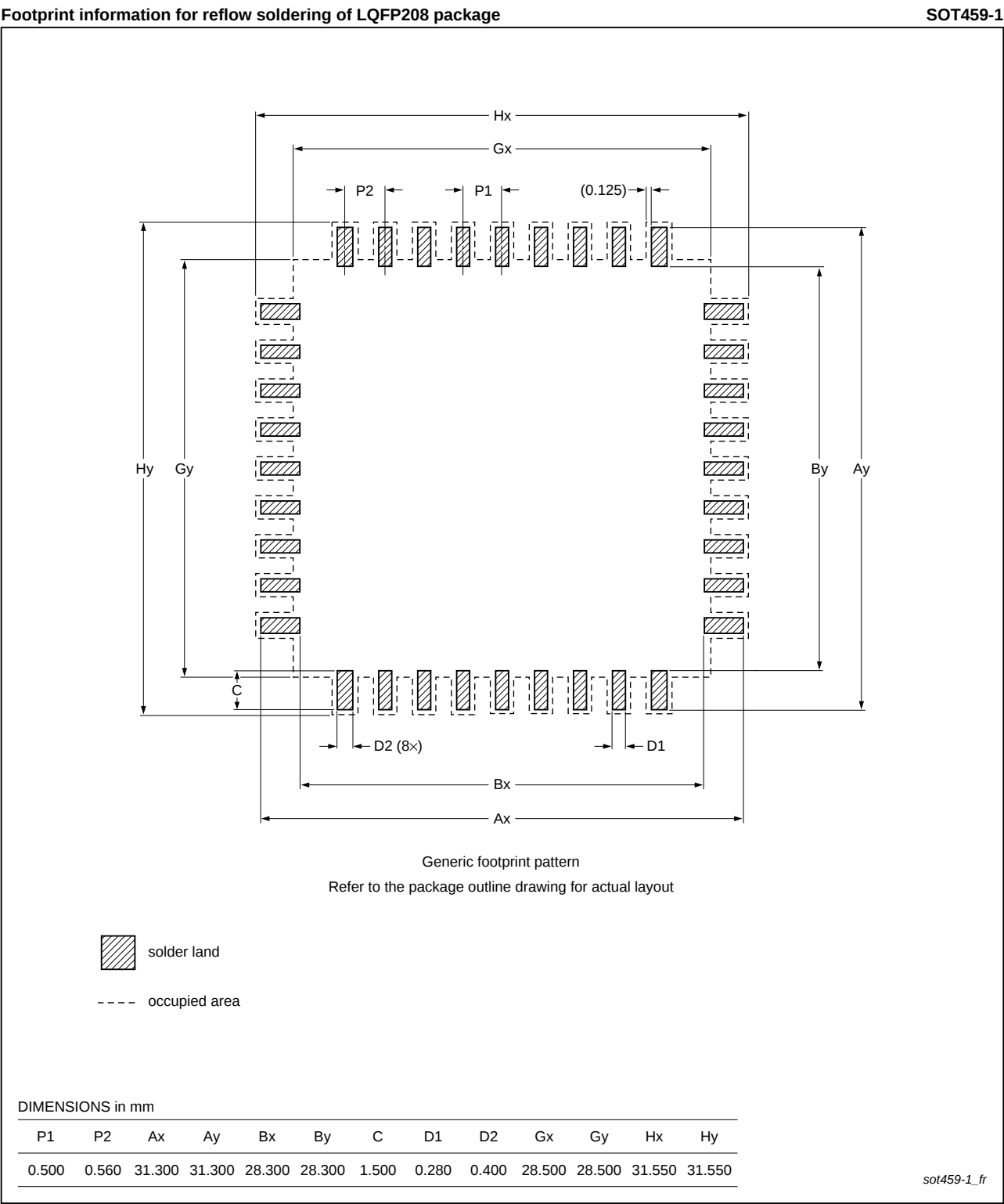
Fig 56. Reflow soldering of the LQFP208 package
