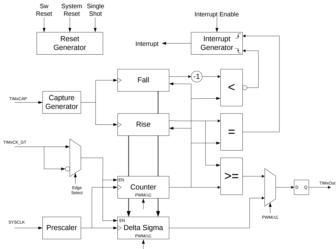
Figure 25: Timer Unit Block Diagram
