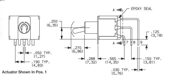
7301MD9AV2BE Vertical Actuation 3PDT
