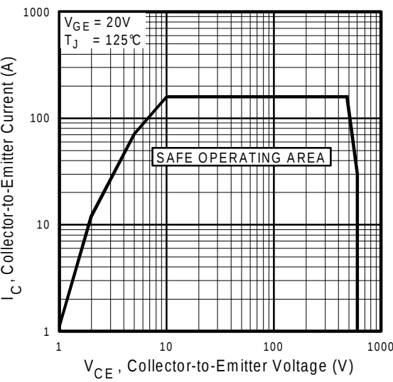
Fig. 12 - Turn-Off SOA
