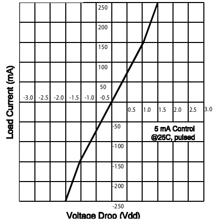
Figure 2. Linearity Characteristics
