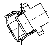
SECTION C-C VERSION 4 (MTP-MTP) SEE NOTE 2
