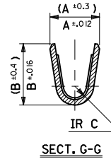
SECT. G-G
