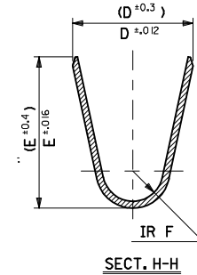
SECT. H-H
