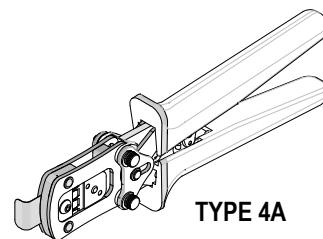
Hand Crimp Tool Order No. 63823-6900
