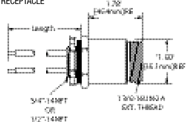
MALE RECEPTACLE
