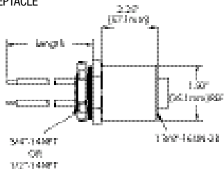
FEMALE RECEPTACLE
