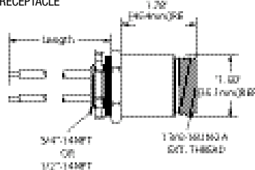
MALE RECEPTACLE
