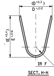
SECT. H-H
