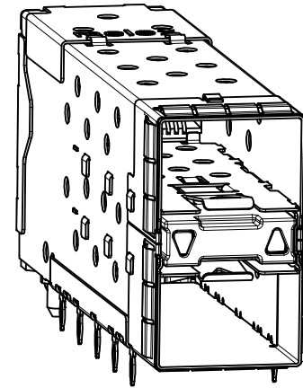
760440003 AND 760445003 WITH OUTER LIGHTPIPER
