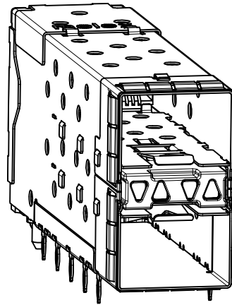
760440001 AND 760445001 WITH INNER AND OUTER LIGHTPIPER
