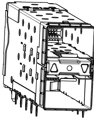
760445004 WITH OUTER LIGHTPIPER
