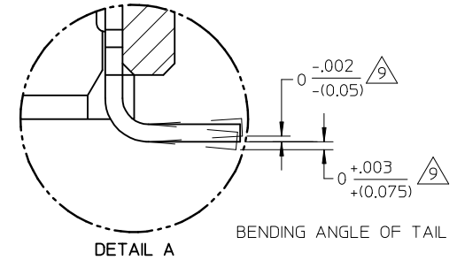
BENDING ANGLE OF TAIL
