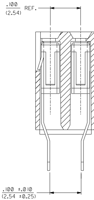
SECTION E-E
