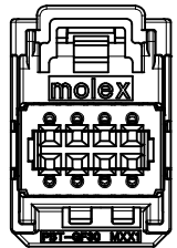
POLARIZATION OPTION C P/N 34729-0082
