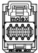
POLARIZATION OPTION B P/N 34729-0081
