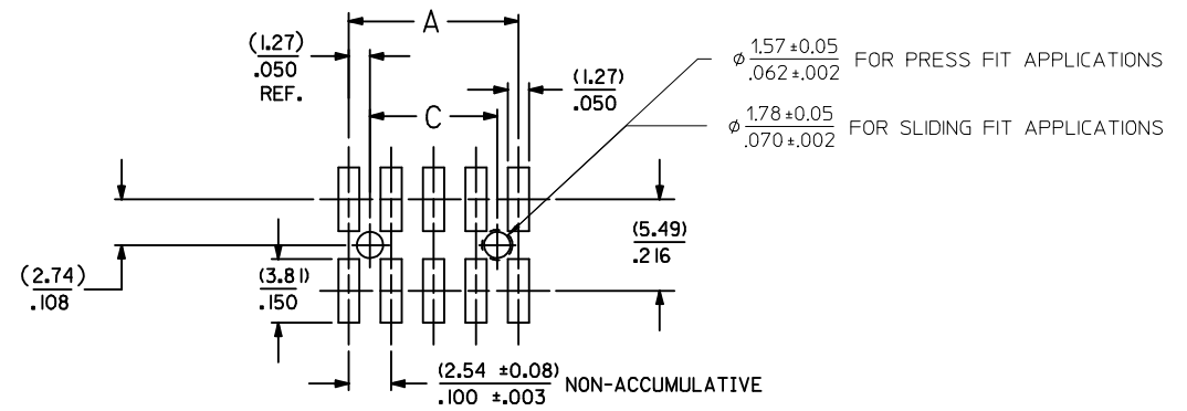
RECOMMENDED P.C. BOARD LAYOUT SCALE: 4:1
