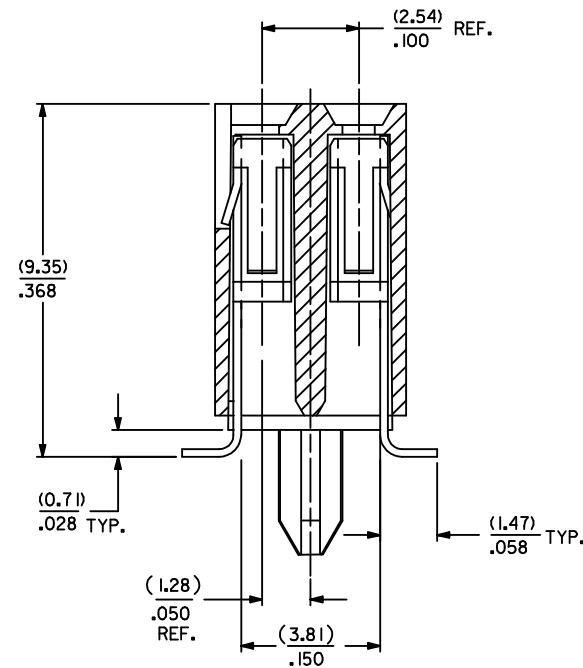
SECTION B-B
