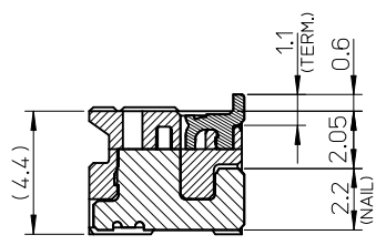
SECTION Z-Z
