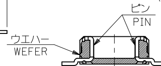
SECT.W-W(LOCK PART)
