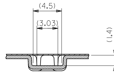
SECTION X-X SCALE 5:1
