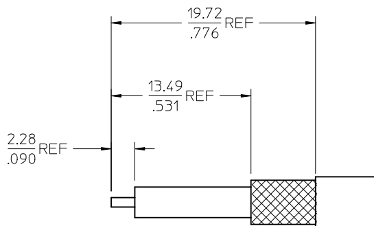
STRIP DIMENSIONS
