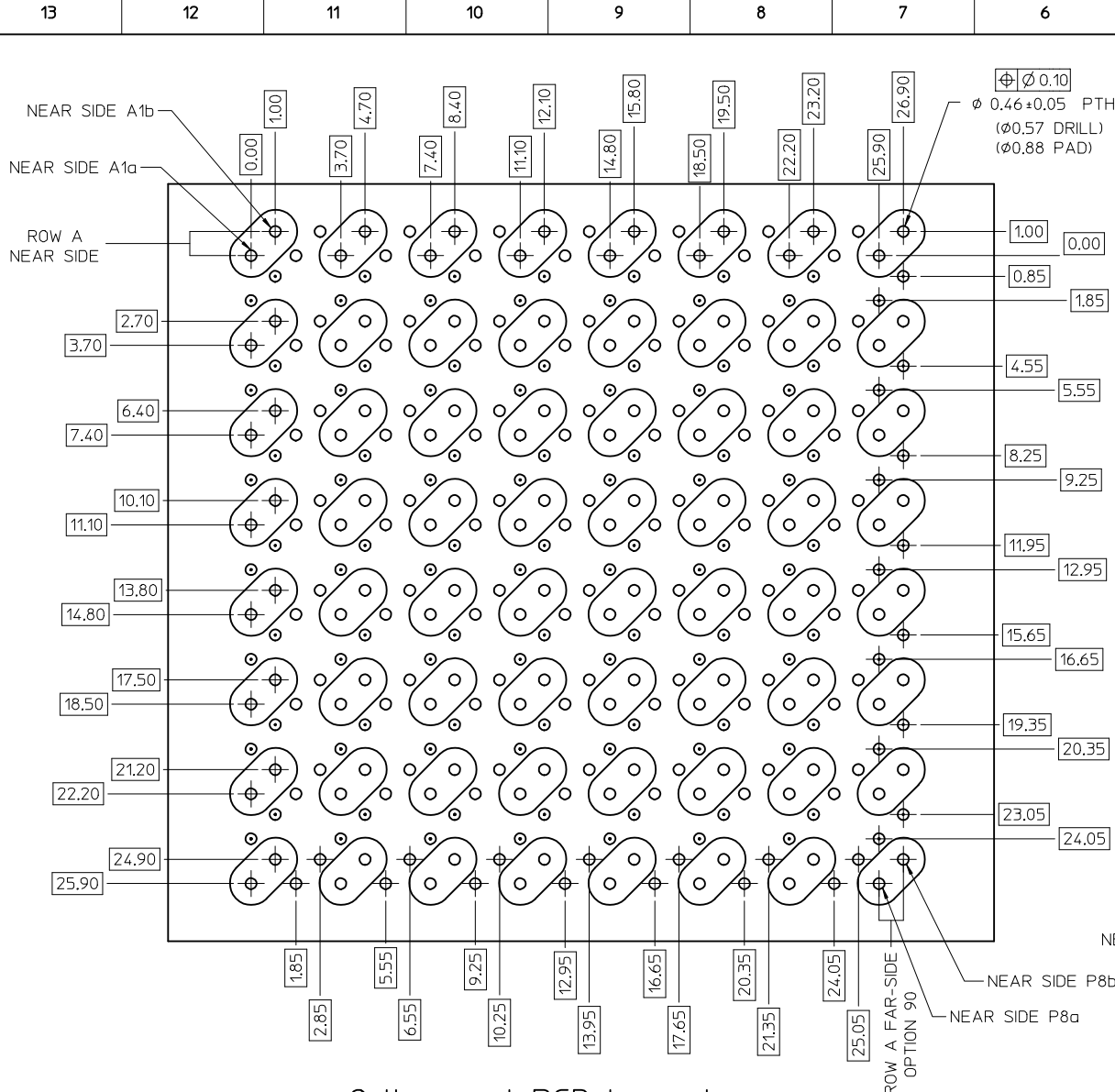
Orthogonal PCB Layout
