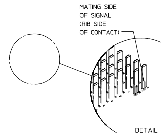
DETAIL SCALE 5:1
