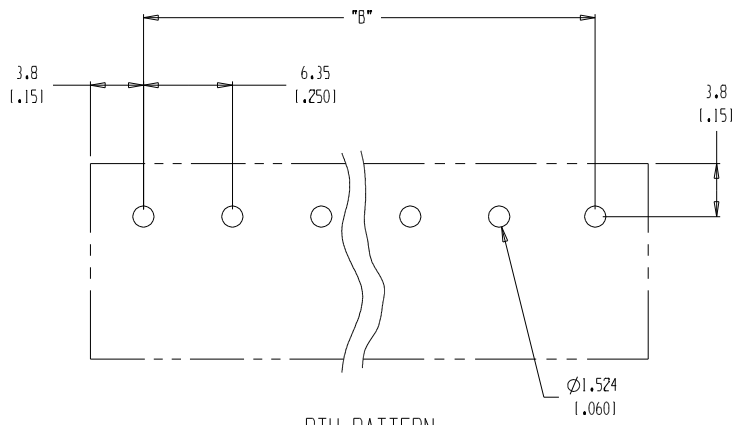
PTH PATTERN
