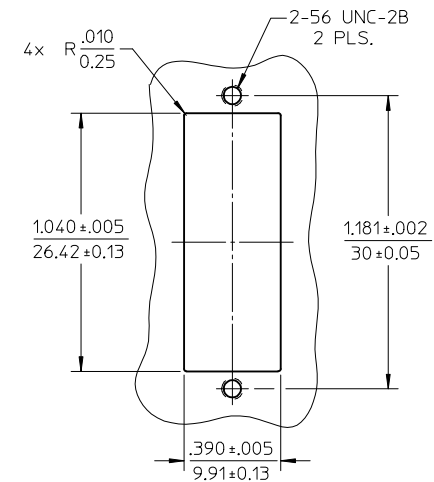
RECOMMENDED MOUNTING PATTERN SCALE 2:1
