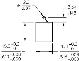
PANEL CUTOUT SCALE 1:1
