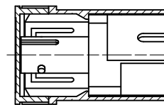
SECTION B-B VERSION 1 (ST-SC) ROTATED 30° CW
