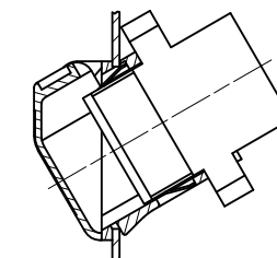
SECTION C-C VERSION 4 (MTP-MTP) SEE NOTE 2
