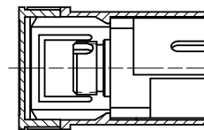
SECTION B-B VERSION 2 (FC-SC) ROTATED 30° CW
