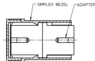
SECTION B-B VERSION 3 (SC-SC) ROTATED 30° CW
