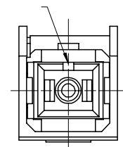
VIEW A VERSION 3 (SC-SC) DOOR REMOVED ROTATED 30° CW
