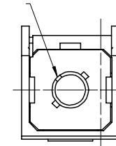
VIEW A VERSION 1 & 2 (KEY LOCATION) DOOR REMOVED ROTATED 30° CW
