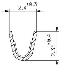
SECT. X-X
