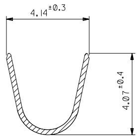
SECT. Y-Y
