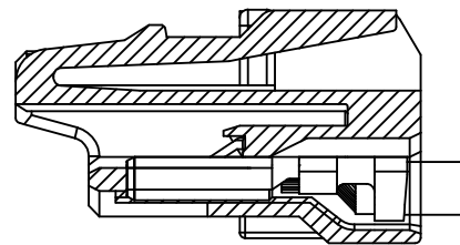
TERMINAL ASSEMBLY DRAWING
