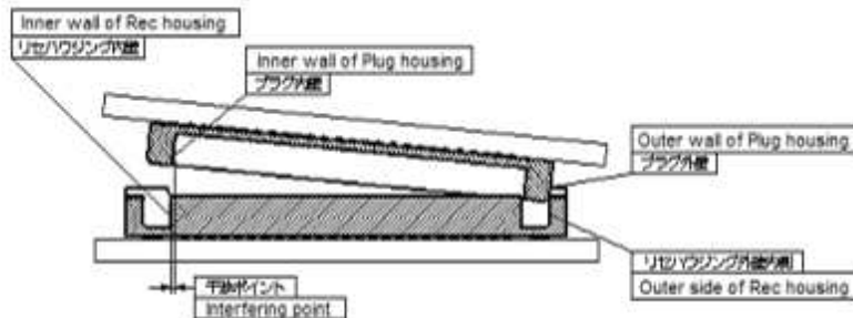
× 図-3 外壁合せによる挿抜 (Not Good) Figure-3 Mating aligning to outer wall of housings (Not Good)
