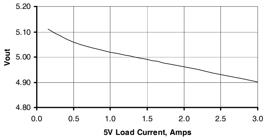
Figure IX. 5.0 V Output Regulation Limits 0.3 A load on \pm 15 V outputs
