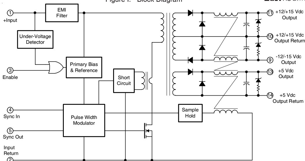
Figure I. Block Diagram
