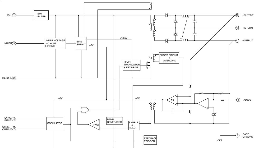
Figure 2. Block Diagram - Dual Output
