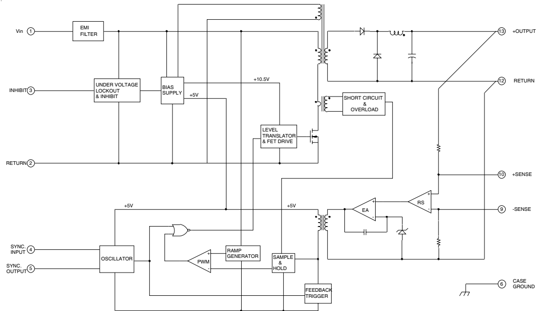
Figure 1. Block Diagram - Single Output
