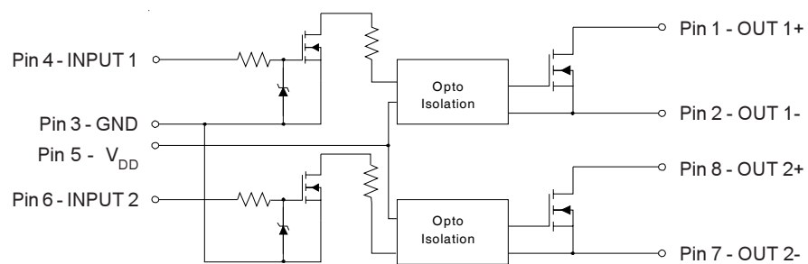
Fig 2: Typical Application
